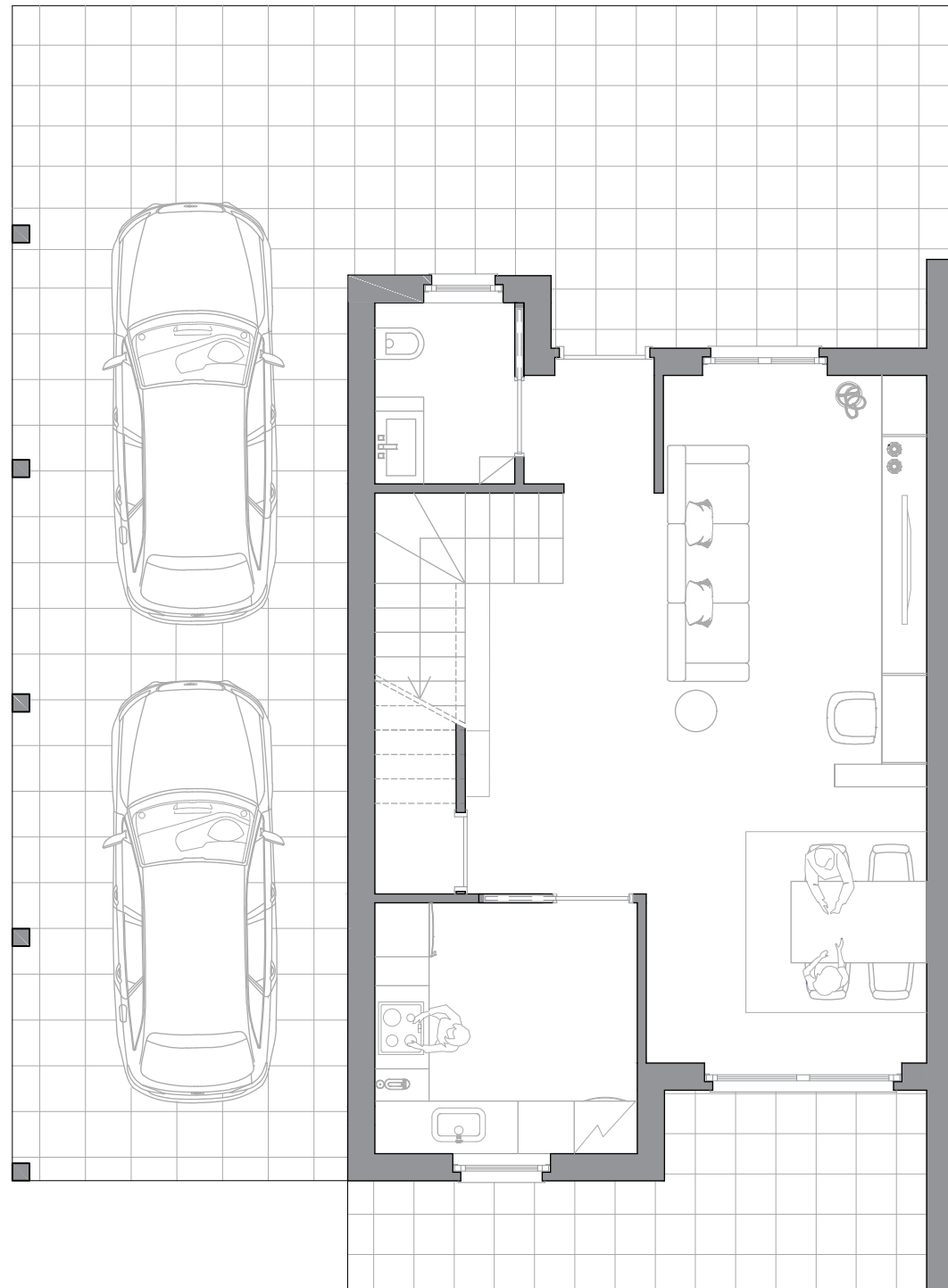
PIANO TERRA
